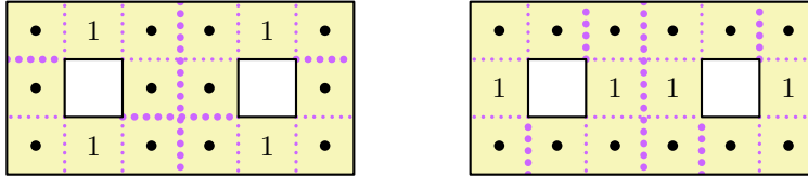
Figure 14: A polyomino that does not fold into a cube.
