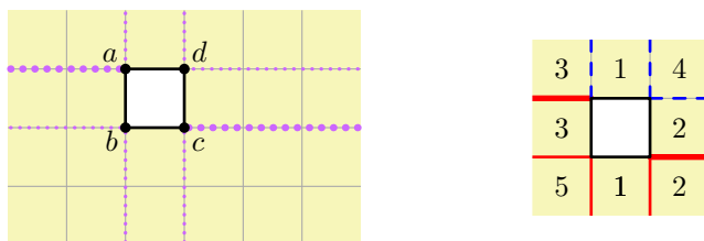
Figure 13: Thinner dotted/purple lines indicate creases folded by \pm 90^\circ , while thicker dotted/purple lines indicate creases folded by \pm 180^\circ . Left: crease pattern around a unit-square hole folding into an L-shape when grid points a and c are mapped to the same corner of \mathcal{C} ; creases shown in purple can be both mountain or valley. Right: numbers indicate the face of the cube in the folded state; mountain folds are shown as red solid lines, and valley folds as blue dashed lines.
