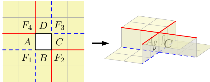
Figure 12: Four edges of a square hole glued together.
