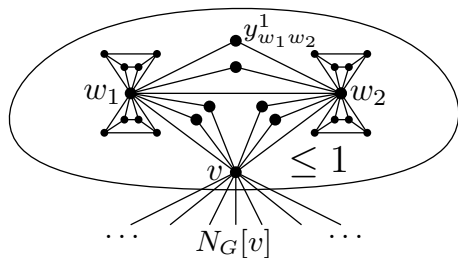
Figure 3: Gadget G_{\leq 1}
