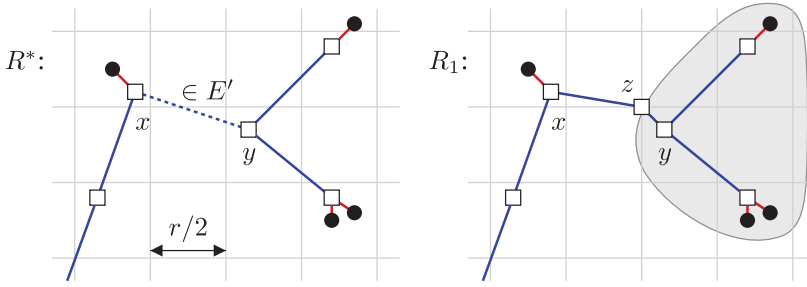
Fig. 11. Construction of R_1 for dense instances. Each edge in the set E' is replaced by a path of length 2. The grey area shows one of the subtrees. The leaf nodes of the subtree are now pinned at points of C_0 , and there are, at most, m internal nodes. Figure 12 shows how we can “pin” the internal nodes of the subtree to points of G .
