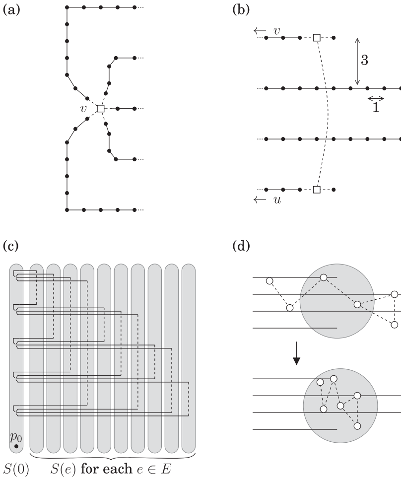
Fig. 6. (a) Vertex gadget for v \in V . (b) Crossover gadget for \{v, u\} \in E . (c) Reduction for K_5 . (d) Normalising a solution, step 1.
