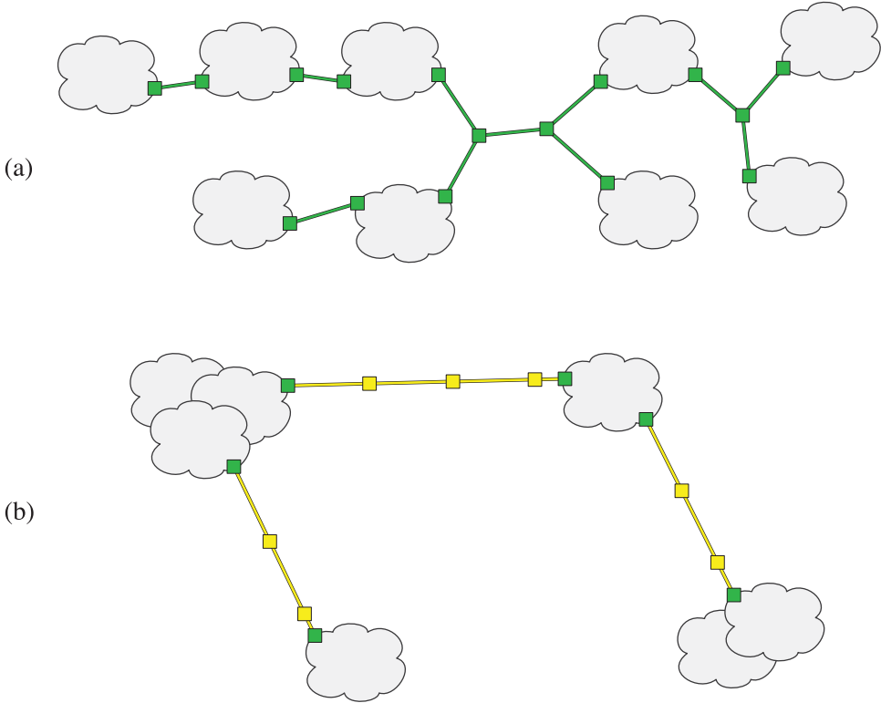
Fig. 4. (a) Green relays connect clouds into clusters – on average, we use at most 2 green relays per cloud. (b) Green (inside clouds) and yellow (outside clouds) relays interconnect the cloud clusters by a spanning tree.
