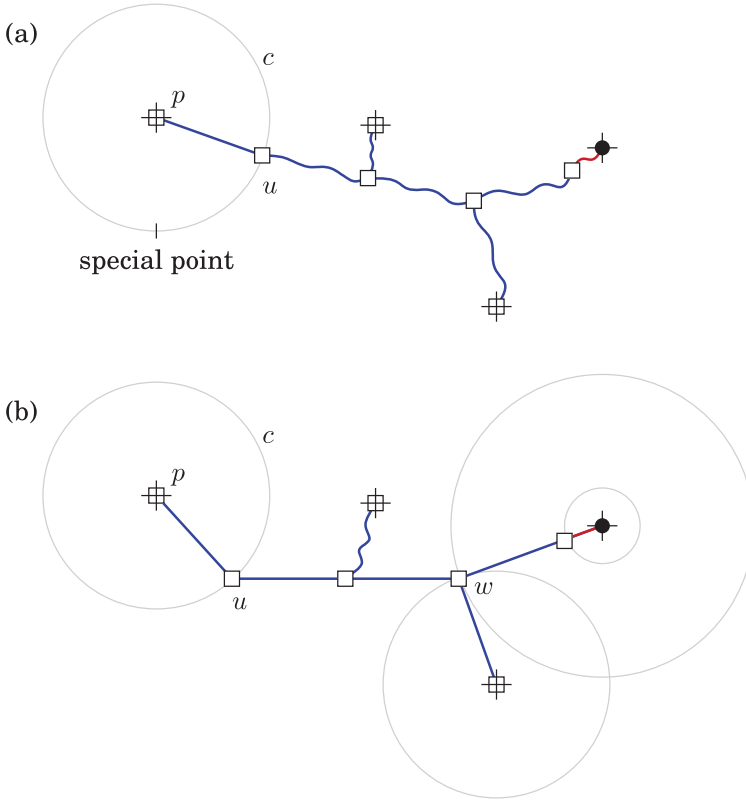
Fig. 12. Pinning a subtree. Black dots are sensors and white boxes are relays. The leaf nodes are pinned at points of C_i . Straight lines denote “taut” edges, that is, red edges of length 1 or blue edges of length r ; other edges are shown with winding lines. (a) We have translated the internal nodes until the edge between a leaf node p and an internal node u becomes taut. Then, we try to slide u along circle c towards the special point. If we succeed, we have pinned u at the special point, which is in C_{i+1} . (b) In this case, we cannot slide u to the special point. However, from the subtree of taut edges, we can find a node w that is now located at a point of C_{i+1} – in this case at the intersection of a circle of radius r + 1 centered at a sensor, and a circle of radius r centered at a pinned relay.
