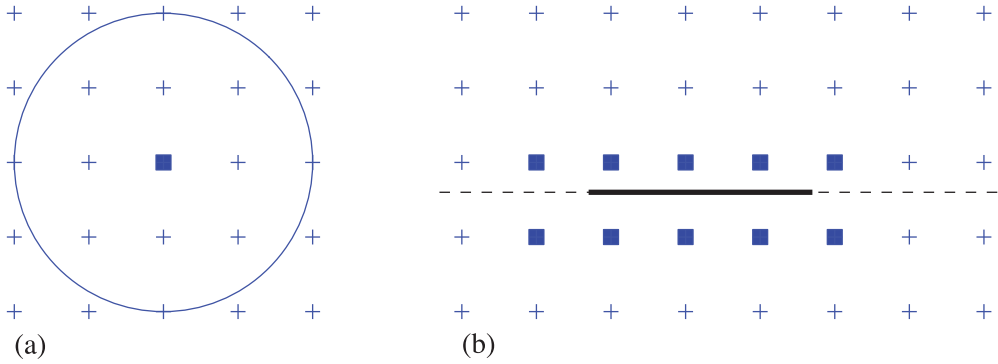
Fig. 10. (a) Regular square grid G_0^{\text{blue}} of spacing r/2 . (b) A relay-dense m -span \sigma_m^{\text{blue}}(\ell) .
