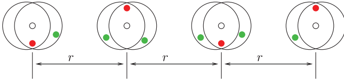
Fig. 7. Unit disks centered on the sensors are shown. The optimum has 1 relay per blob (hollow circles). Our algorithm may place 1 red relay in every blob plus 2 green relays in (almost every) blob.
