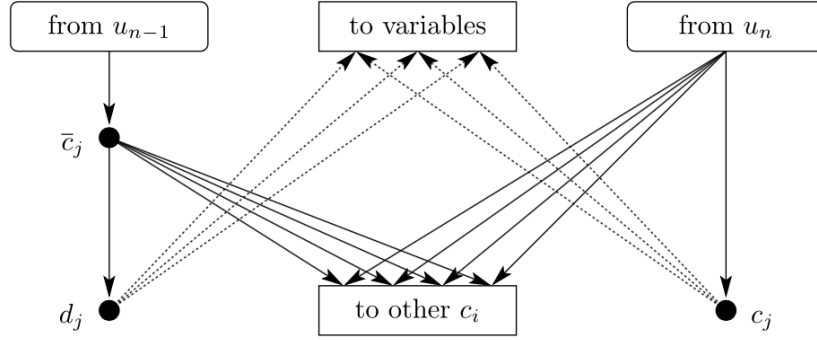
Fig. 3. A clause gadget: The player picks a clause by moving to a clause selector vertex \bar{c}_j , which is connected to all clause nodes c_k for k \neq j . This forces the adversary to move to c_j in order to avoid being caught prematurely. Then the player moves to d_j , catching the adversary after he moves to one of the three variable vertices corresponding to the clause c_j . The adversary wins if and only if that vertex already carries a load of 1, i.e., if the corresponding variable satisfies the clause.
