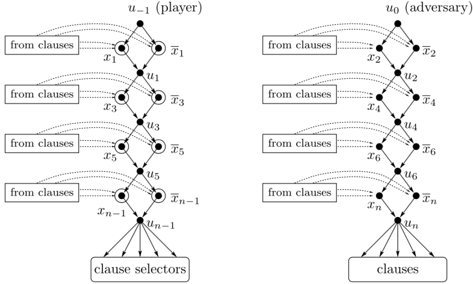
Fig. 2. The variable gadget: The player chooses a truth setting for the odd variables by running from u_{-1} to u_{n-1} , while the adversary chooses a truth setting for the even variables by running from u_0 to u_n . Note that initially, the odd-numbered vertices carry a load of 1 (indicated by circles), while all other vertices start out with a load of 0.
