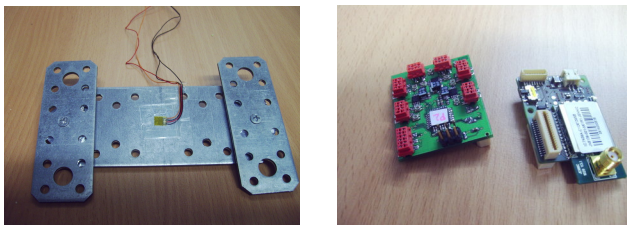
(a) A single load sensor. (b) Amplifier and iSense node.
