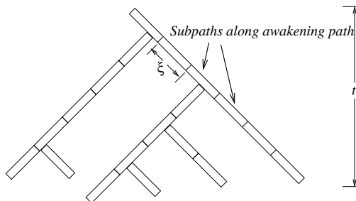
Figure 7: The awakening tree is partitioned into heavy paths, each of which is partitioned into subpaths of length \xi .
