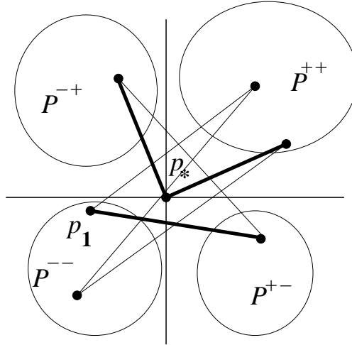
Figure 3: Getting an optimal tour for odd n , when the median is in P .
