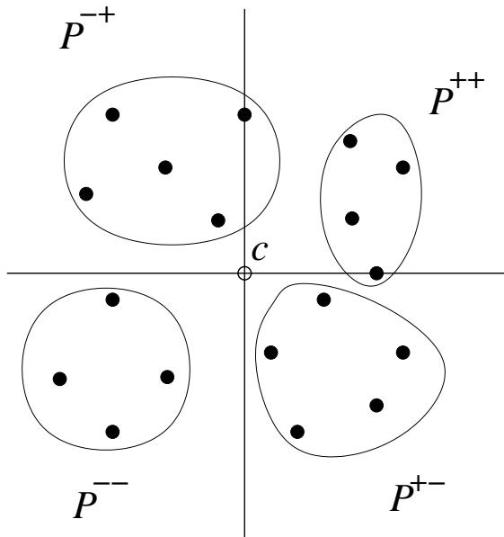
Figure 1: The four quadrants and their point sets.
