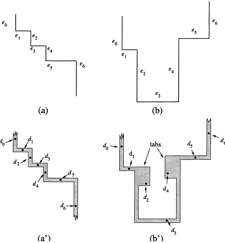
Fig. 3. Pieces to build the annulus for representing a variable: (a) A "stair-case" sequence of edges, e_0, e_1, \dots, e_6 . (a') A representing set of rectangles r_0, r_1, \dots, r_6 , and their dots. (b) A "U-turn" sequence of edges, e_2, e_3, e_4 , and their neighbors. (b') A representing set of regions; also shown are the modifications ("tabs") added to rectangles r_2 and r_4 , and the position of all dots.
