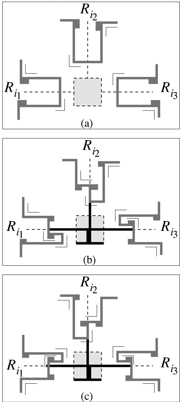
Fig. 4. (a) Three different annuli, for variables x_{i_1} , x_{i_2} , x_{i_3} , with U-turns close to the vertex for clause (x_{i_1} \vee \overline{x_{i_2}} \vee x_{i_3}) ; the indicated L-shapes correspond to the truth assignments of x_{i_1} , x_{i_2} , or x_{i_3} that would satisfy c . (b) Local modifications to annuli R_{i_1} , R_{i_2} , R_{i_3} near their U-turns. (c) The same operations for clause (\overline{x_{i_1}} \vee x_{i_2} \vee x_{i_3}) .
