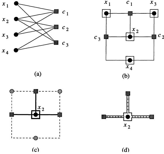
Fig. 1. (a) The bipartite graph G_I corresponding to the 3SAT instance (x_1 \vee x_2 \vee \overline{x_3}) \wedge (\overline{x_2} \vee x_3 \vee x_4) \wedge (\overline{x_1} \vee x_2 \vee \overline{x_4}) . (b) A planar rectilinear embedding of G_I . (c) The "star" of edges adjacent to a variable node, x_2 . (d) A "loop" constructed from the star of edges.
