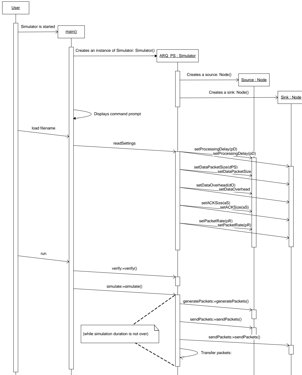
Fig 2: Sequence diagram showing sequence of operations inside “load” and “run” command
