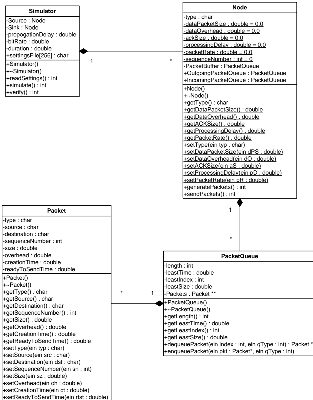
Fig 1: Simulator Structure: class diagram
