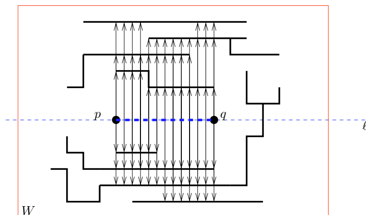
FIG. 3.1. Subsegment pq \subset \ell is 3-dark; its length is charged to the 3 levels of E that lie above it and the 3 levels of E that lie below it.
