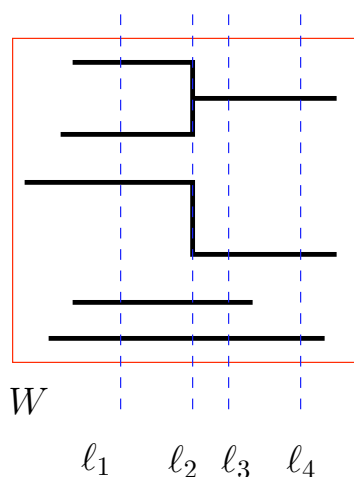
FIG. 2.2. The vertical cuts \ell_1, \ell_2, \ell_3, \ell_4 are 3-perfect (also m -perfect, for m \geq 4 ). The cut \ell_4 is also 2-perfect (but not 1-perfect).
