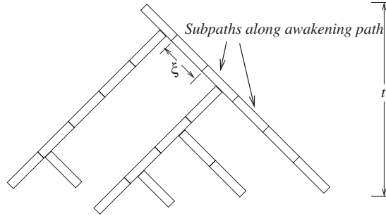
Fig. 7. The awakening tree is partitioned into heavy paths, each of which is partitioned into subpaths of length \xi .
