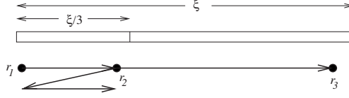
Fig. 8. Robot r_1 awakens the subproblem (r_1, r_3) by first awakening r_2 , the last robot (if any) before distance \xi/3 . Robot r_2 is then in charge of awakening (r_1, r_2) before returning to its original position. Robot r_1 then awakens (r_2, r_3) .
