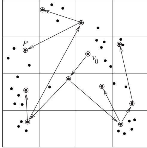
Fig. 9. PTAS for geometric instances. Rescale so that all robots lie in a unit square. Look at the m -by- m grid of pixels, where m = O(1/\epsilon) . Consider an enumeration over a special class of wake-up trees on a set P of representative points, one per occupied pixel.
