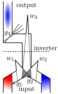
(f) Or gadget, mixed input.
