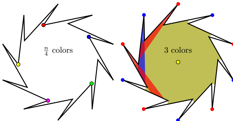
Figure 1: An example polygon with n = 20 vertices. A minimum-cardinality guard cover with n/4 guards requires n/4 colors (left) while a minimum-color guard cover has n/2 + 1 guards and requires only 3 colors (right).
