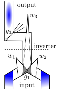
(g) Or gadget, uniform input.
