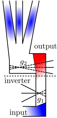
(e) Multiplexer gadget.
