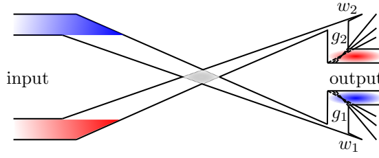
(c) Crossing gadget. \mathcal{V}(w_1) \cap \mathcal{V}(w_2) indicated in gray.
