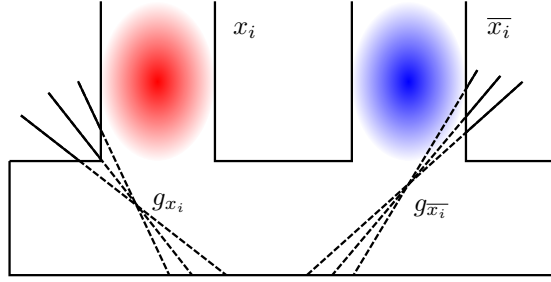
(a) Variable gadget.
